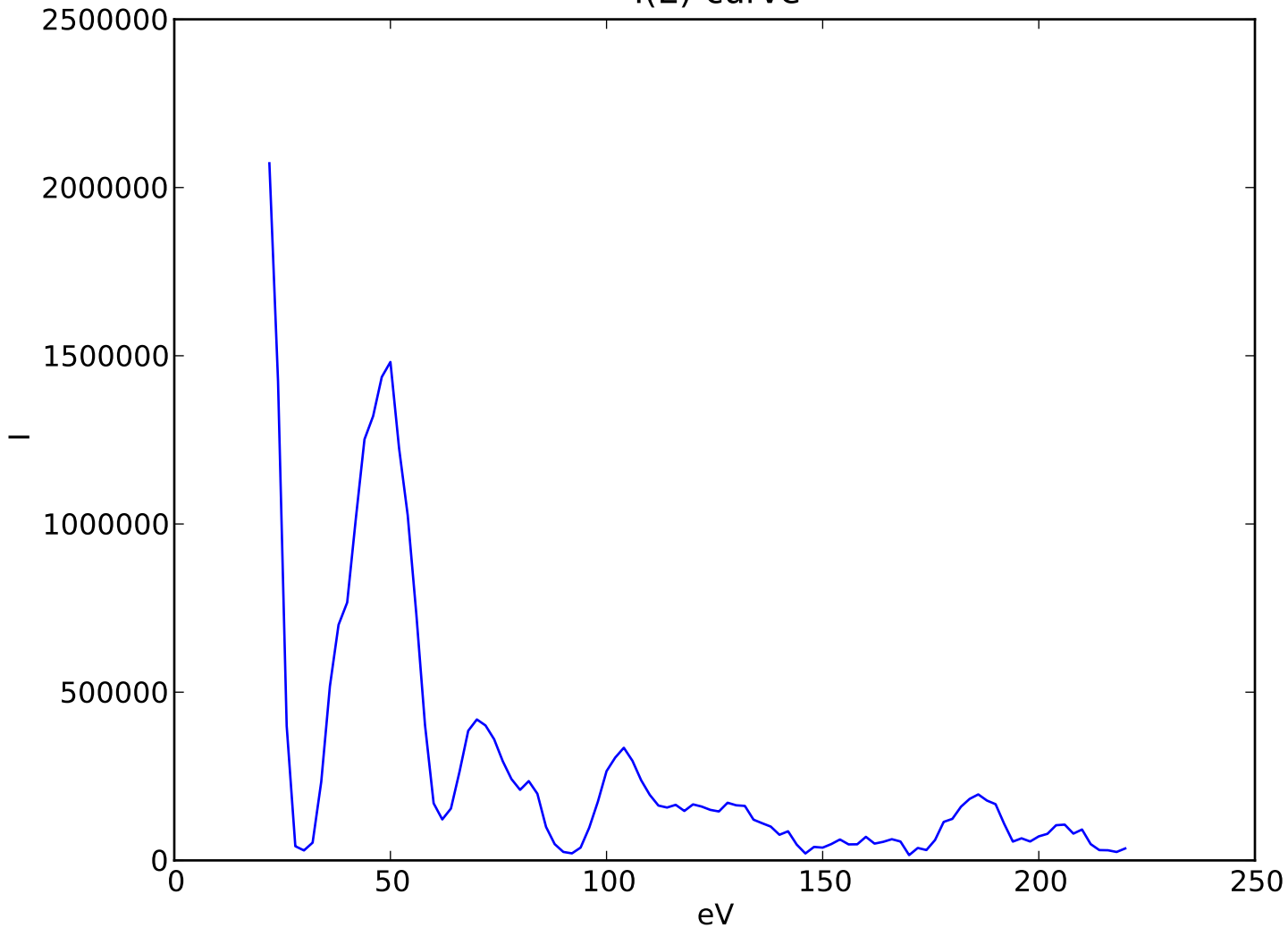
I(E)-curve
