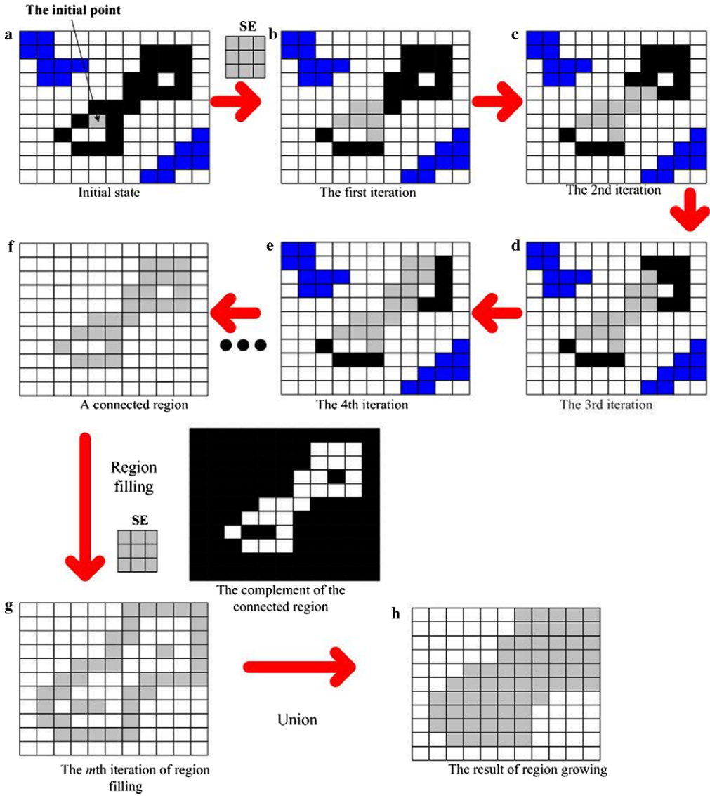
Fig. 3. An example of region growing method.
